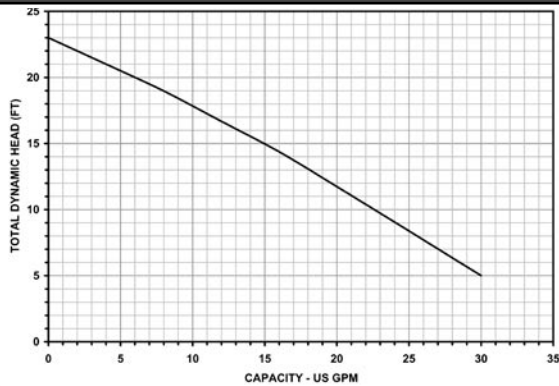
Performance Chart
